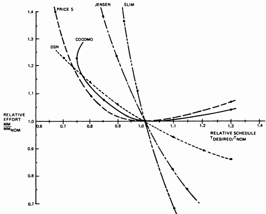
Fig. 5. Comparative effort-schedule tradeoff relationships.
