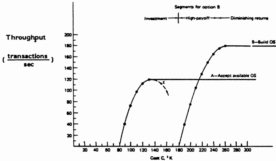
Fig. 2. Cost-effectiveness comparison, transaction processing system options.
