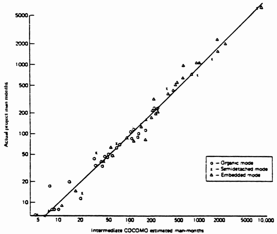
Fig. 7. Intermediate COCOMO estimates versus project actuals.
