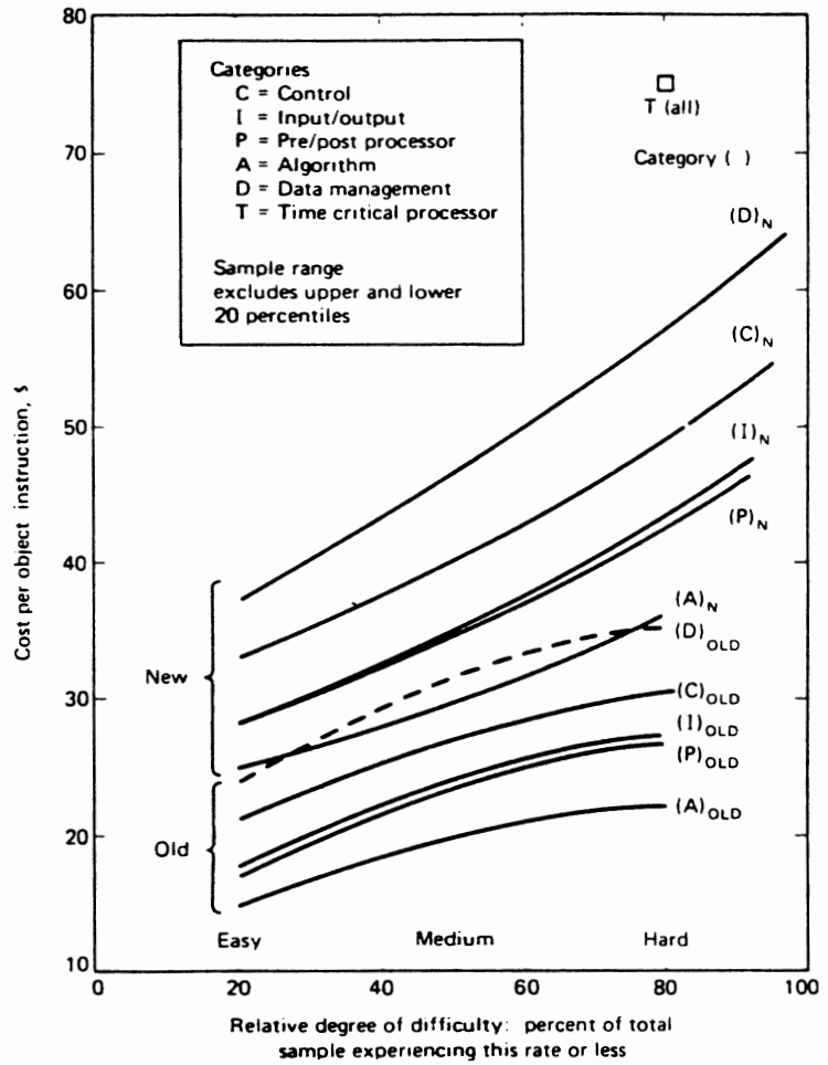
Fig. 4. TRW Wolverton model: Cost per object instruction versus relative degree of difficulty.
