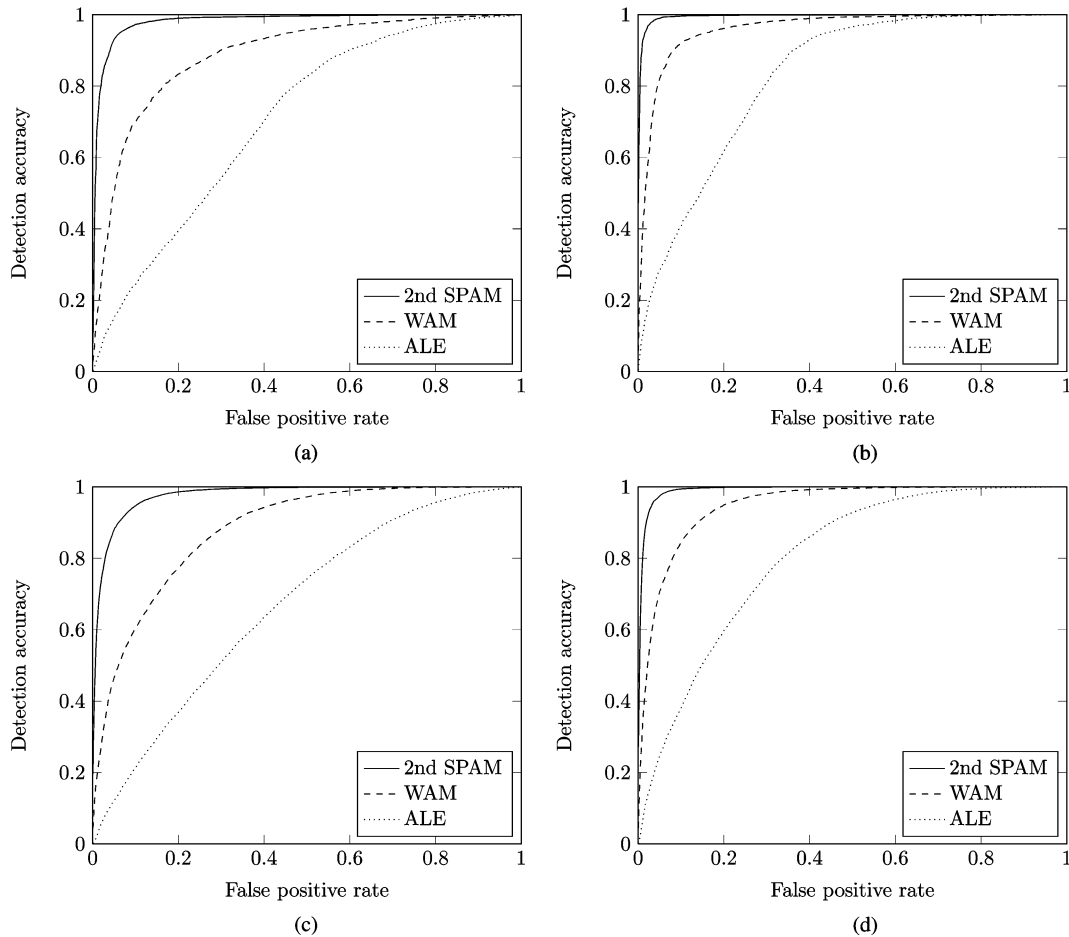
Fig. 4. ROC curves of steganalyzers using second-order SPAM, WAM, and ALE features calculated on CAMERA and JOINT databases.
