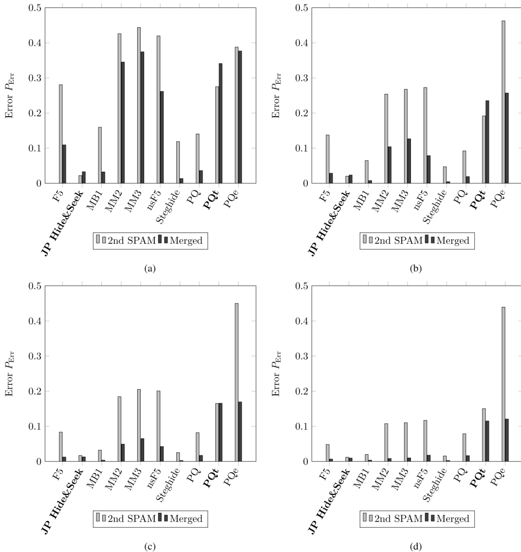
Fig. 5. Error rates P_{\text{Err}} of steganalyzers employing the second-order SPAM features with T = 3 and the Merged features.
