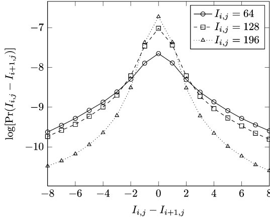
Fig. 2. Probability \Pr(I_{i,j} - I_{i+1,j} | I_{i,j}) (horizontal cuts of the graph shown in Fig. 1) for I_{i,j} = 64 , I_{i,j} = 128 , and I_{i,j} = 196 in 8-bit grayscale images estimated from approximately 10 700 images from the BOWS2 database (see Section IV for more details about the database).
