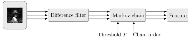
Fig. 3. Schema of extraction of SPAM features.
