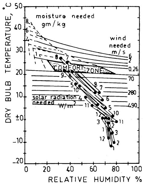
Figure 16. Climatic data plotted new bioclimatic charts of various towns.
