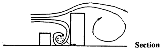
Figure 46. Air flow pattern around buildings of different height.
