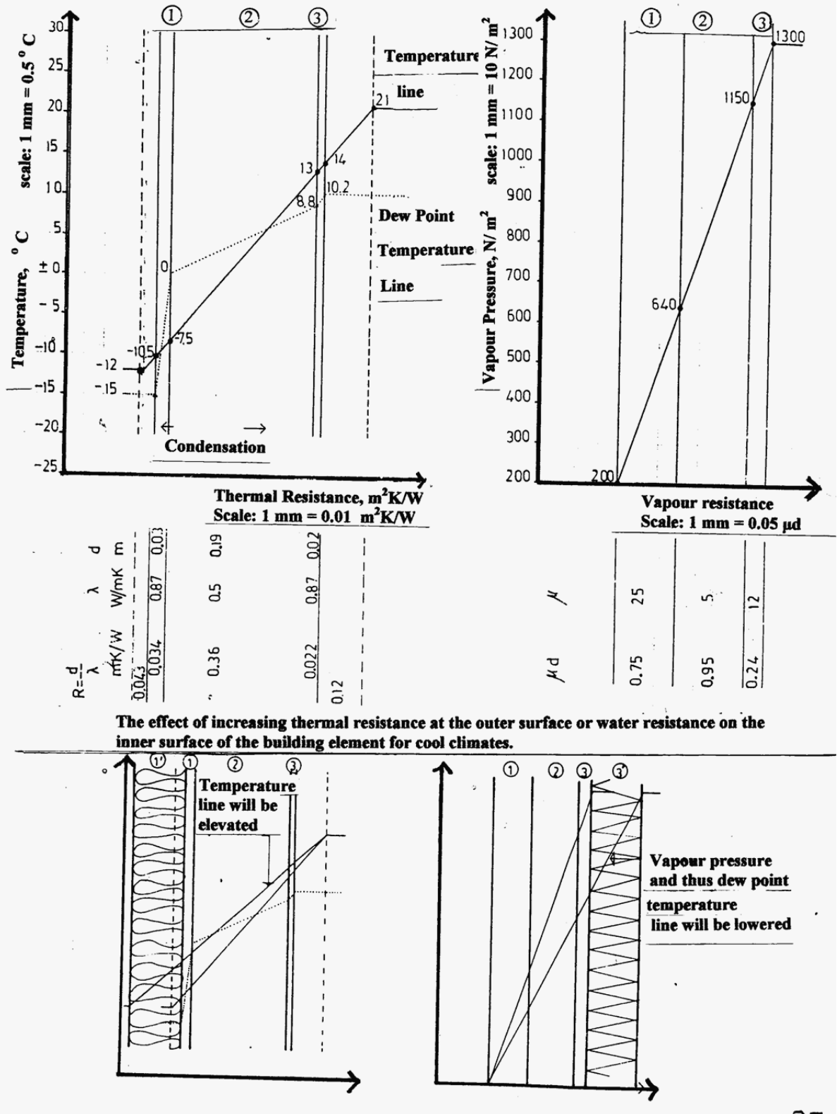
Figure 26. An example of condensation control.
