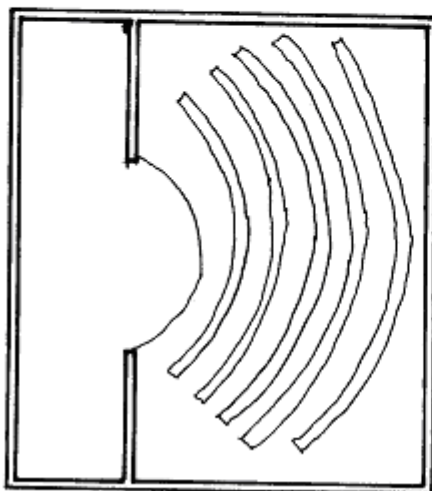
FIGURE 1.21 . Design of sound reflectors (In wide auditoriums reflectors are only used on ceilings not at the side walls).
