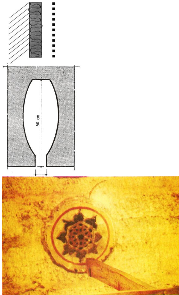
FIGURE 1.14. Large earthenware jars used by Mimar Sinan at the domes of some mosques. (Kayılı, 1989).
