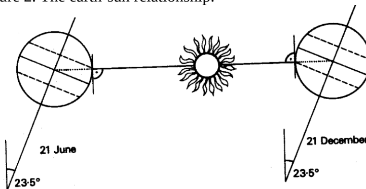
Figure 2. The earth-sun relationship.
