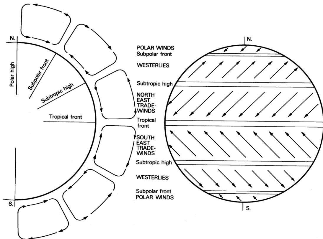
Figure 7. Predominant global winds.
