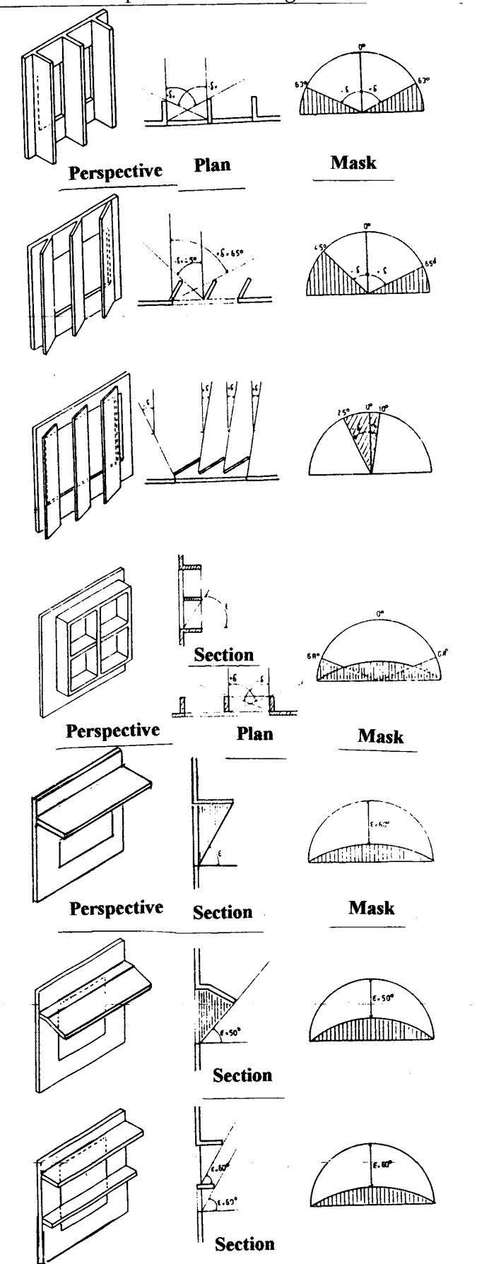
Figure 28. Some examples of the shading devices and shadow masks.
