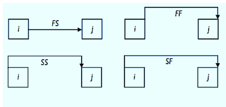
Figure 5.2.2 (b): Relationship between activities
