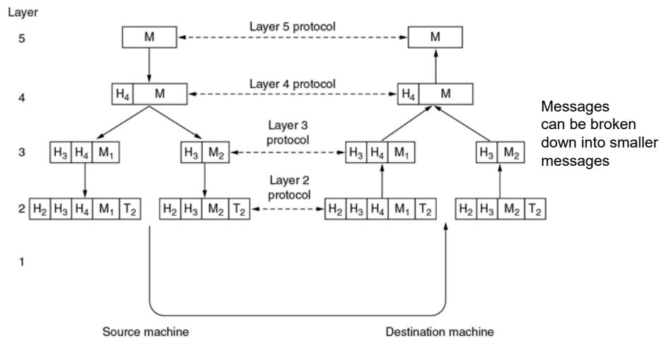
Encapsulation/decapsulation in an example 5-layer architecture 31
