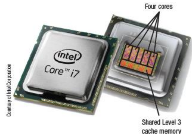
FIGURE 2-13 CPUs. CPUs today typically have multiple cores.
